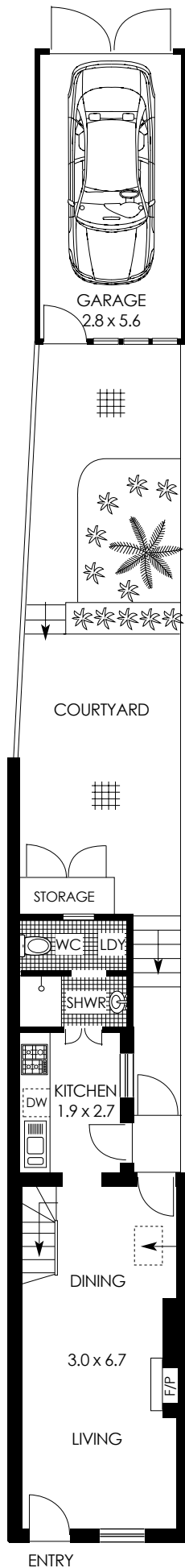
GROUND FLOOR PLAN
